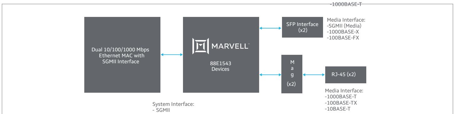
Fig 2. Dual-port SGMII (System) to Copper/SGMII/Fiber with AutoMedia
