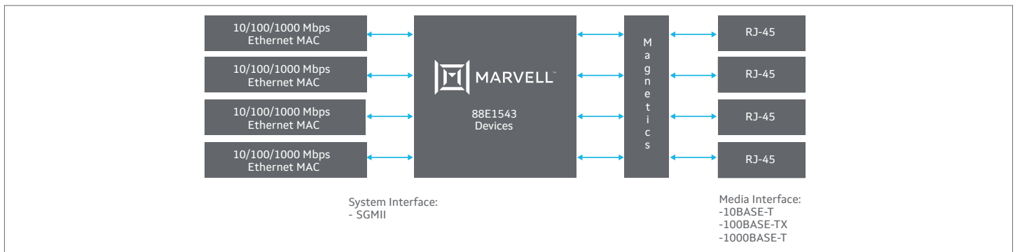
Fig 1. SGMII to Copper Application
